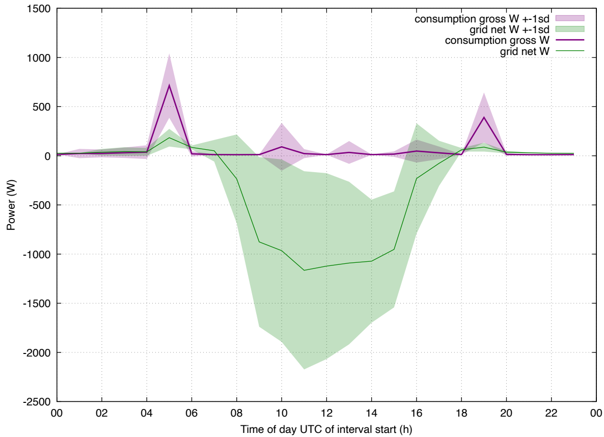
Load Profile: 202604 eddi-hph4 all
