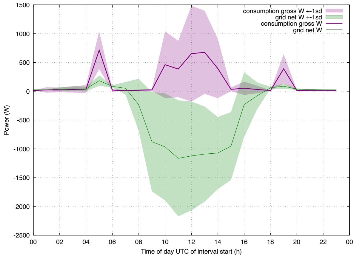
Load Profile: 202604 eddi-ehet all
