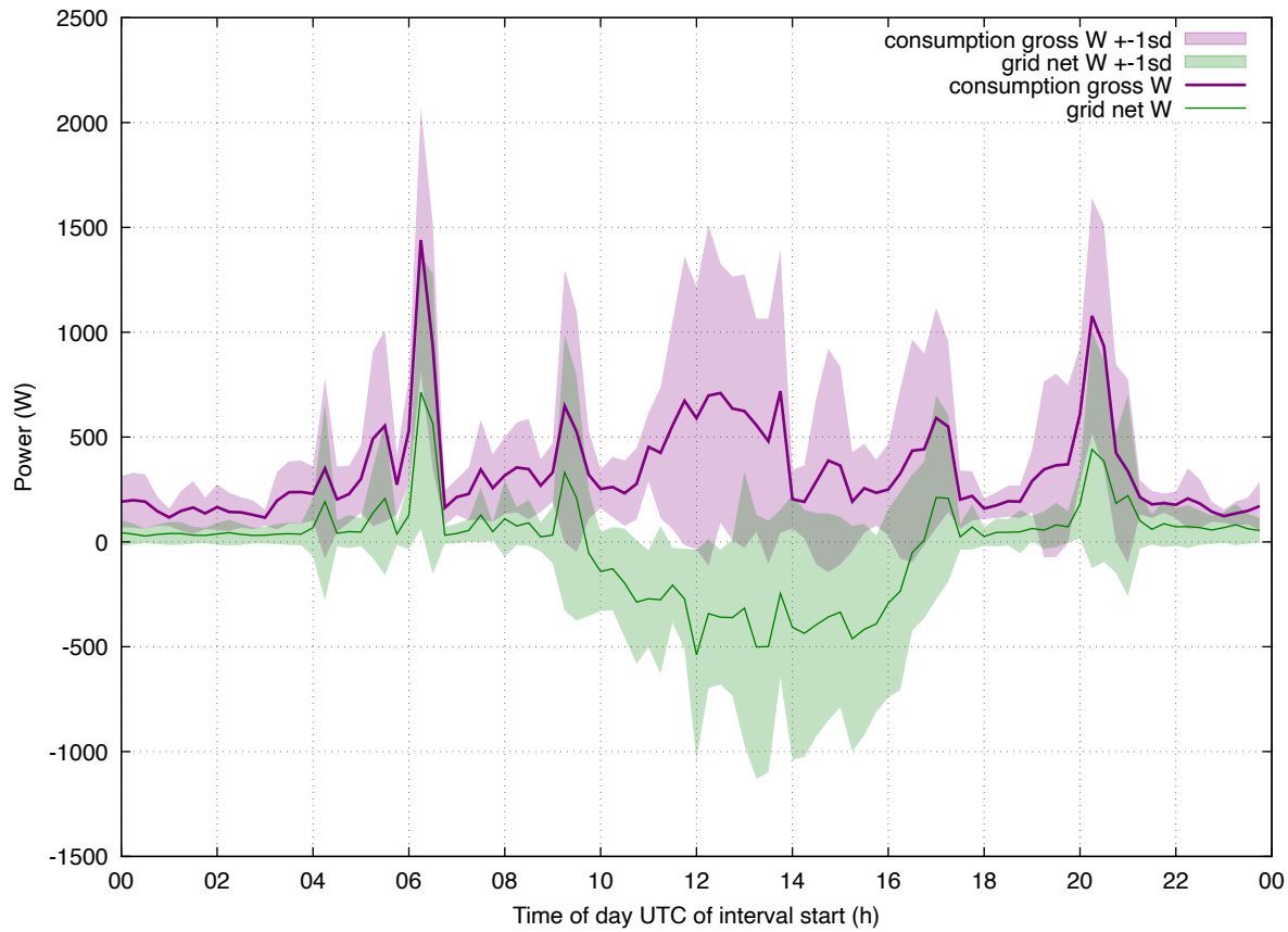
Load Profile: 202603 enphase weekend
