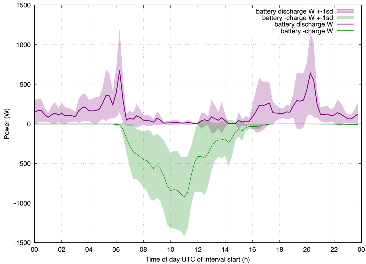
Load Profile: 202603 enphase-batt weekend
