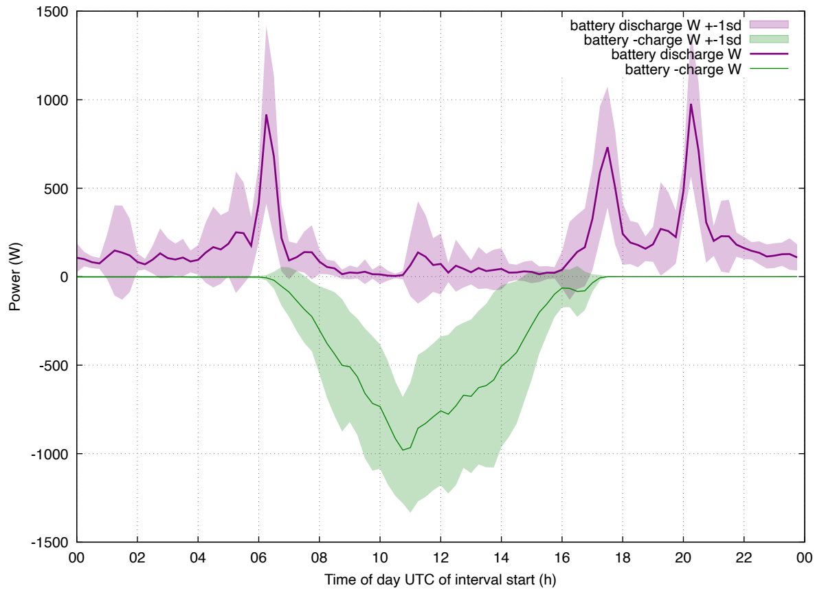
Load Profile: 202603 enphase-batt weekday
