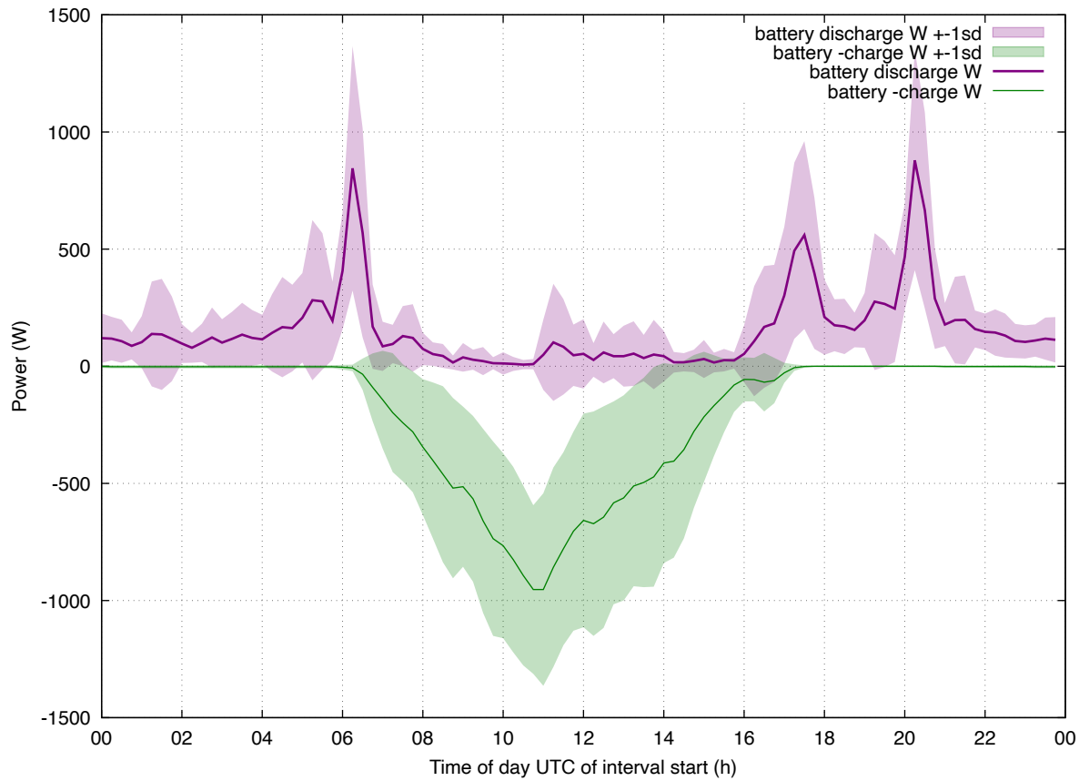
Load Profile: 202603 enphase-batt all
