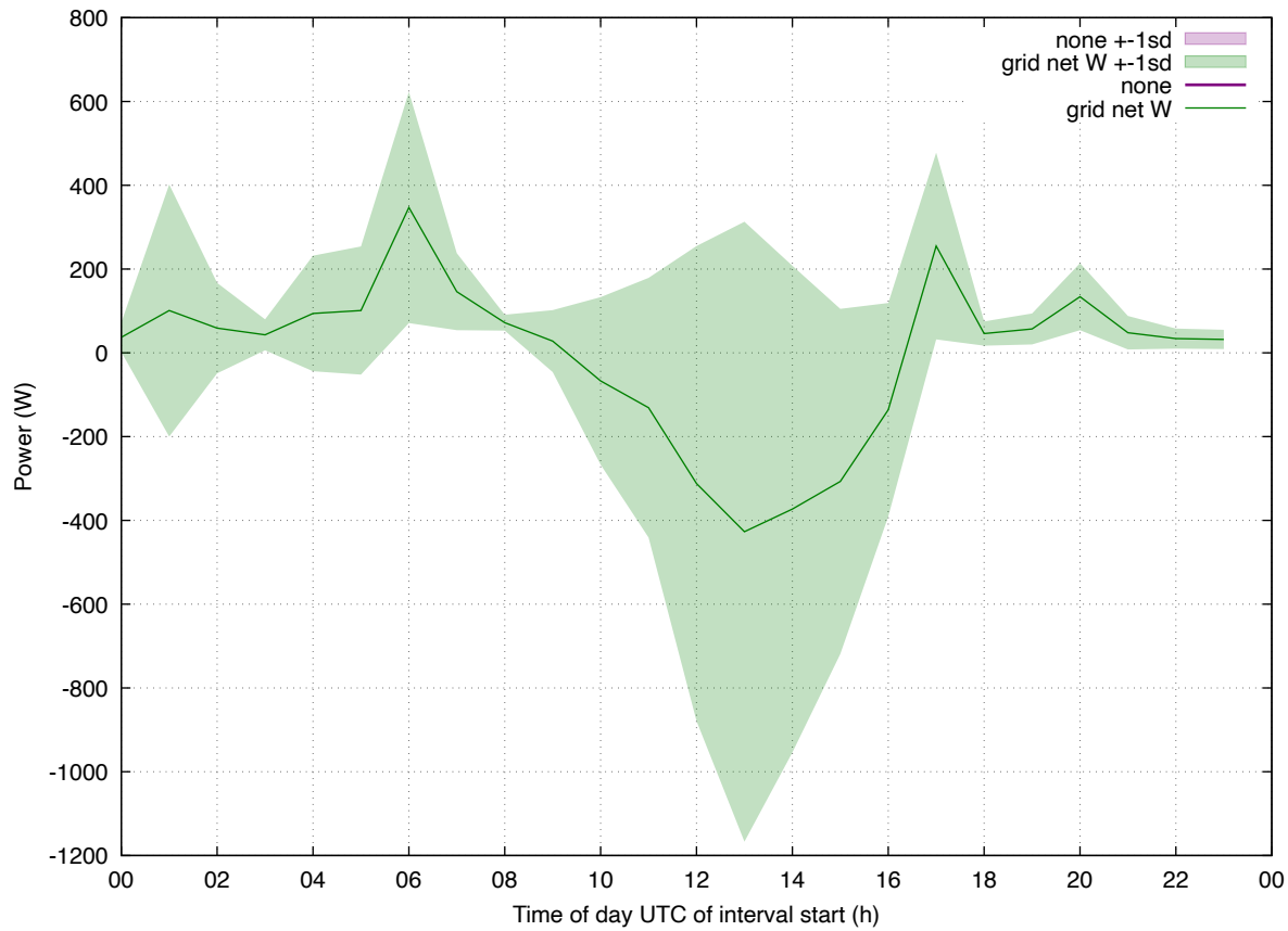
Load Profile: 202603 eddi weekday
