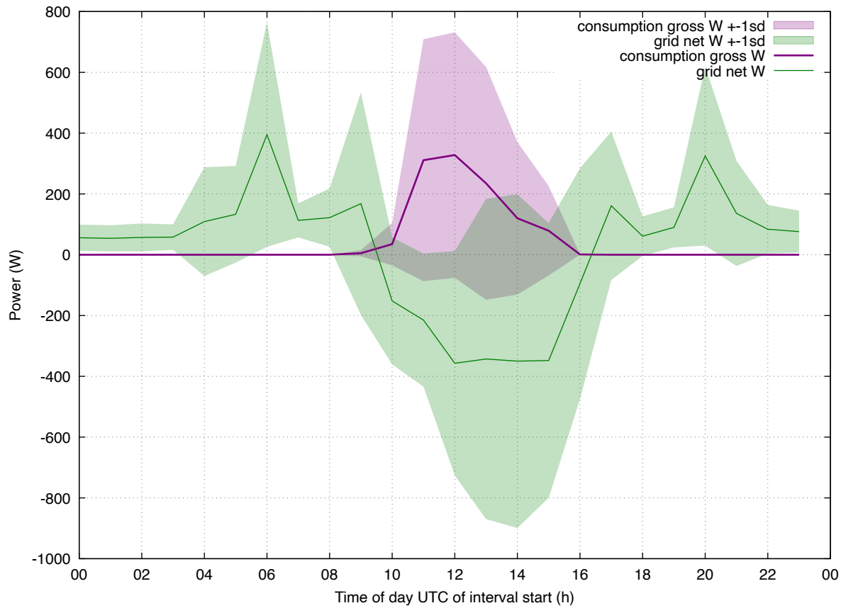
Load Profile: 202603 eddi-ihet weekend
