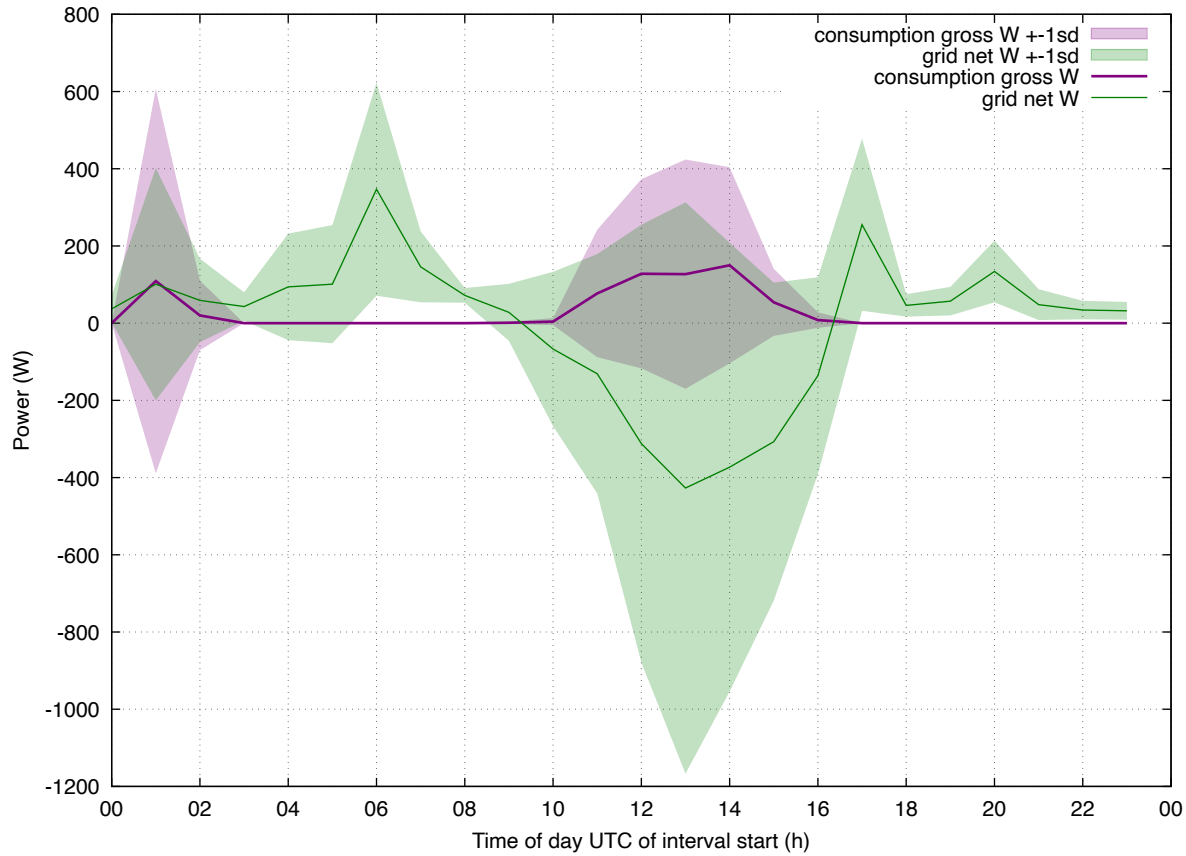
Load Profile: 202603 eddi-ihet weekday
