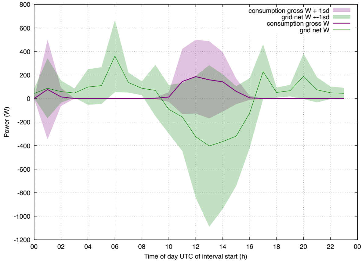
Load Profile: 202603 eddi-iheat all
