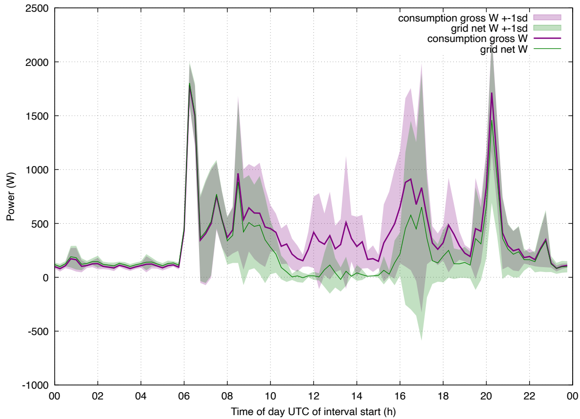
Load Profile: 202602 enphase weekend
