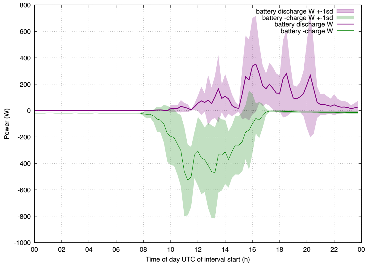
Load Profile: 202602 enphase-batt weekend
