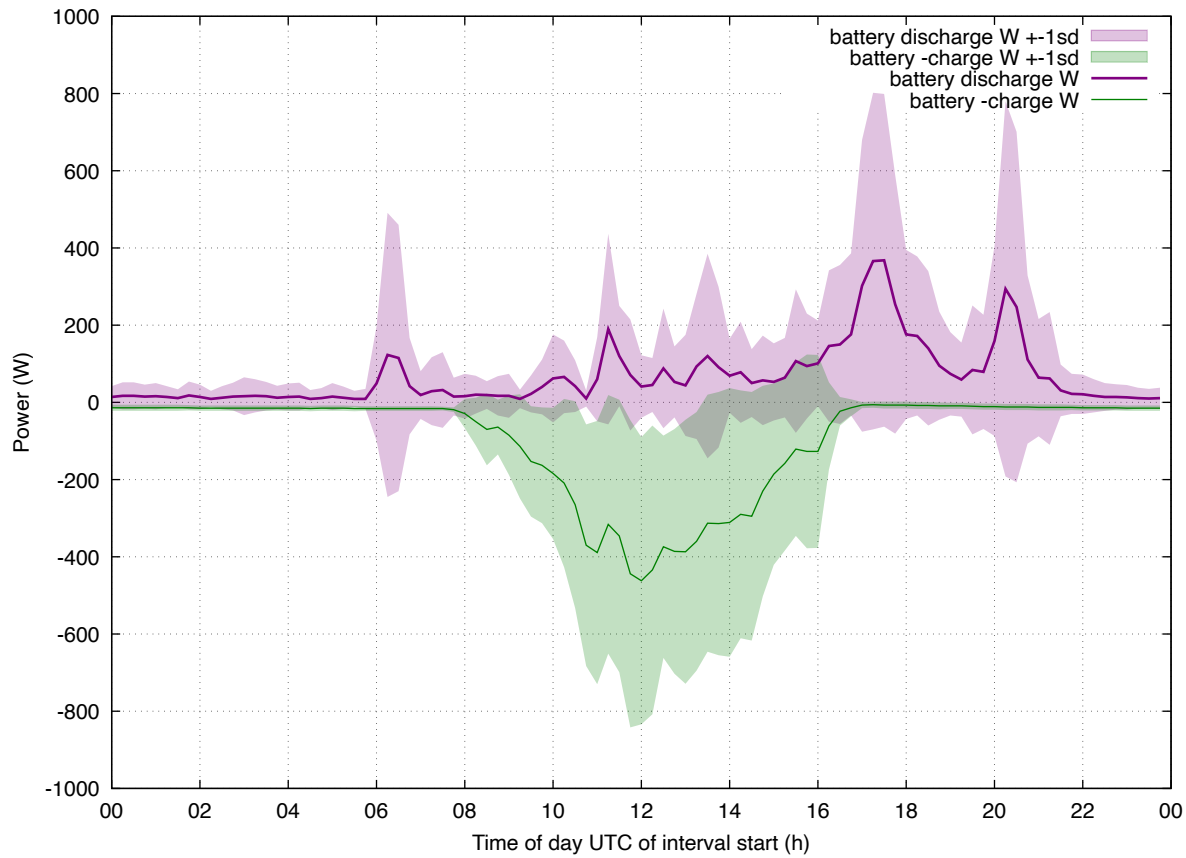
Load Profile: 202602 enphase-batt weekday
