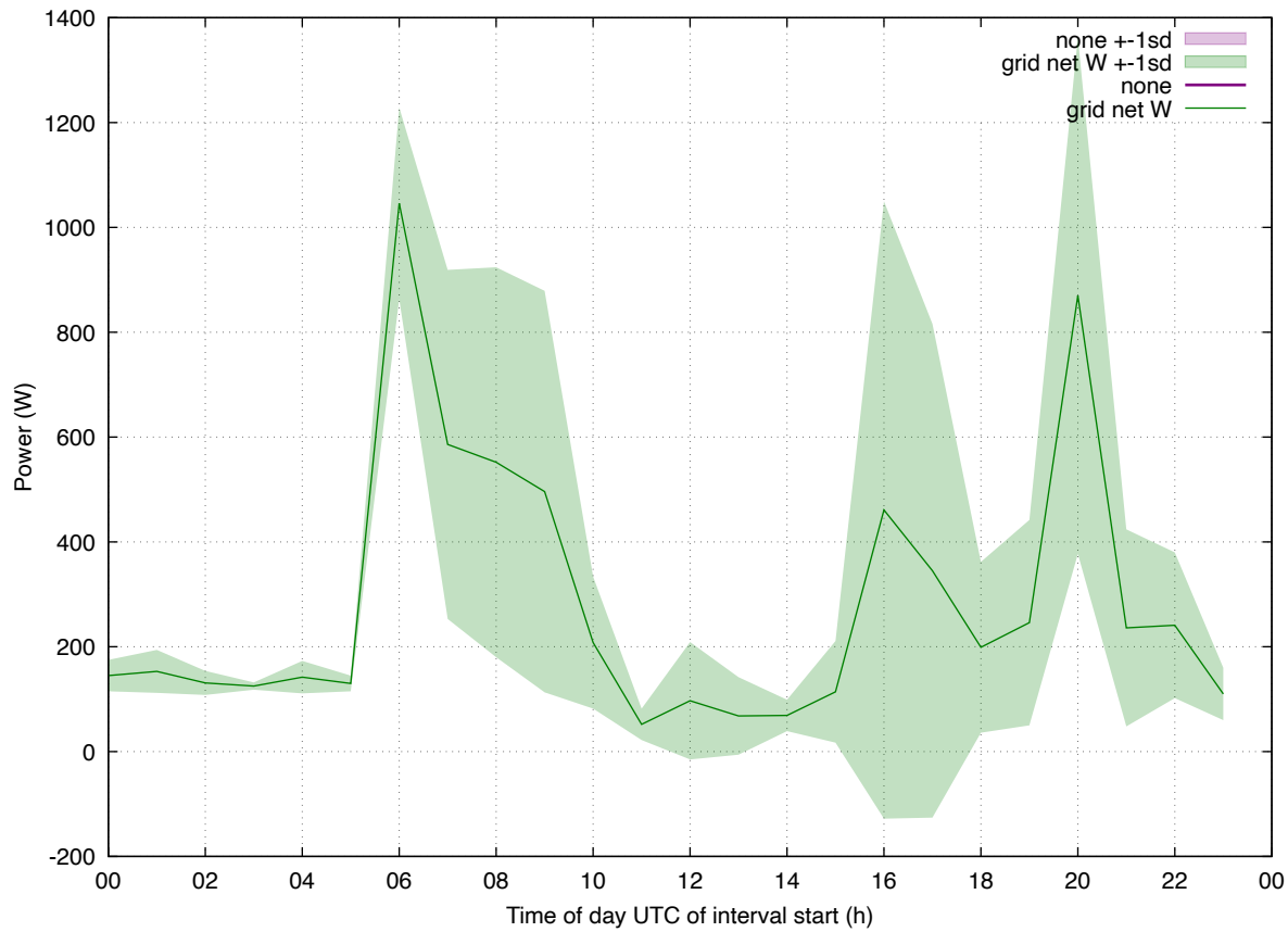
Load Profile: 202602 eddi weekend
