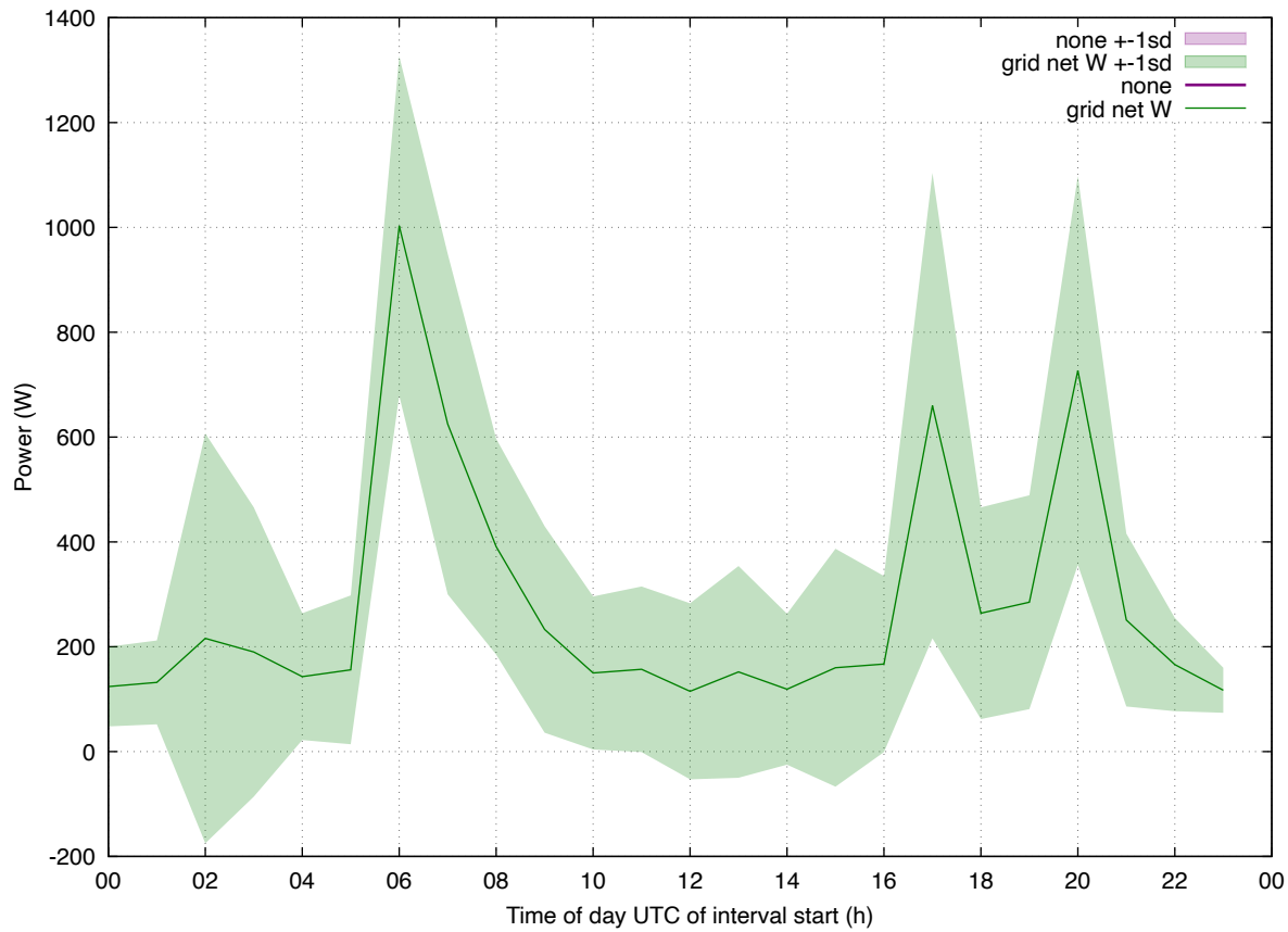
Load Profile: 202602 eddi weekday
