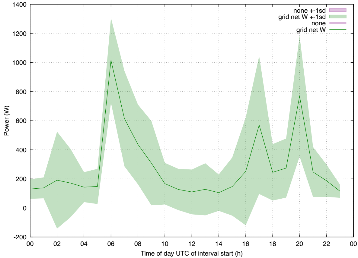
Load Profile: 202602 eddi all
