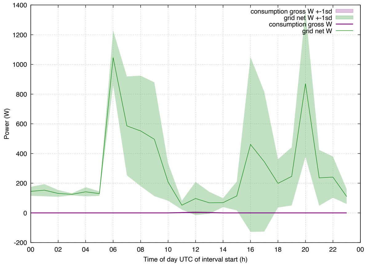
Load Profile: 202602 eddi-iheat weekend
