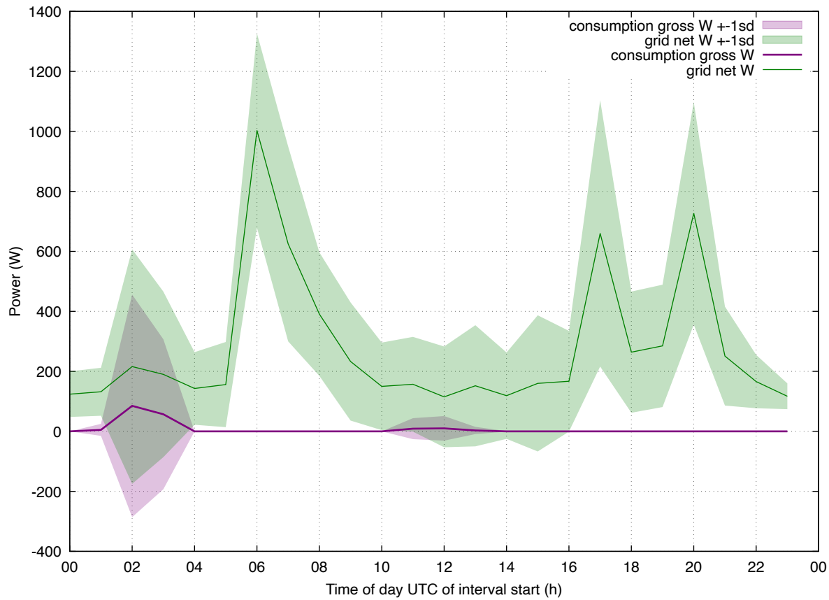
Load Profile: 202602 eddi-iheat weekday
