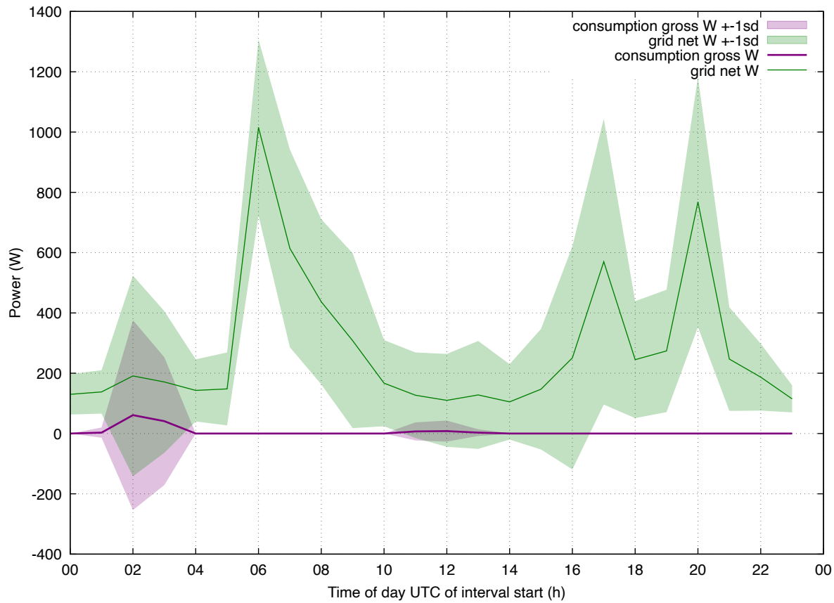
Load Profile: 202602 eddi-iheat all
