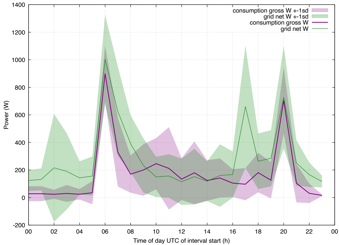
Load Profile: 202602 eddi-hph4 weekday
