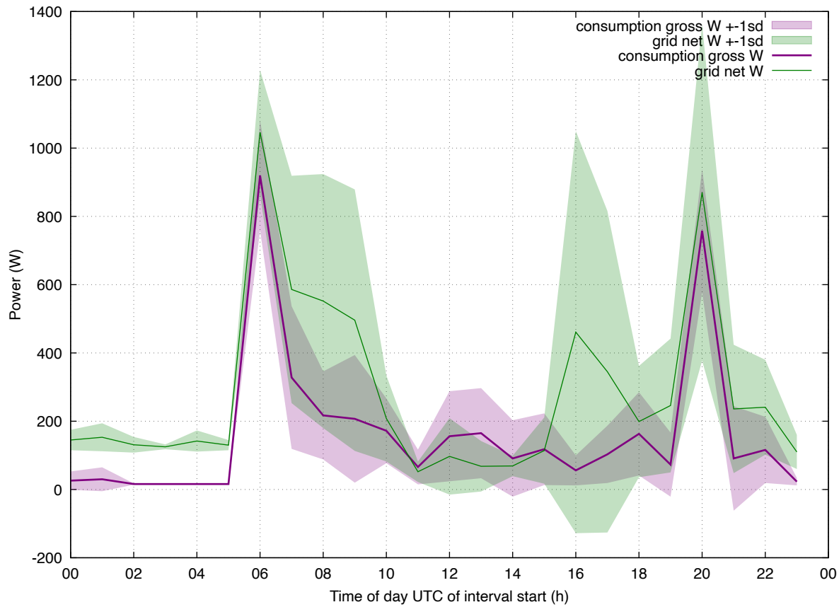
Load Profile: 202602 eddi-eheat weekend
