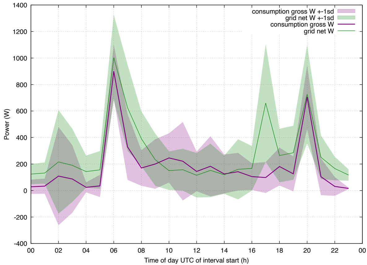
Load Profile: 202602 eddi-eheat weekday
