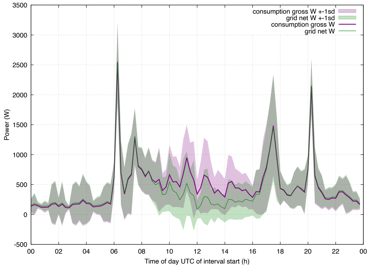
Load Profile: 202601 enphase weekday
