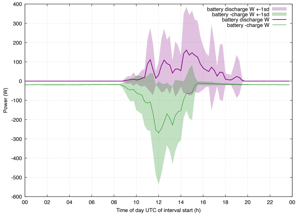
Load Profile: 202601 enphase-batt weekday
