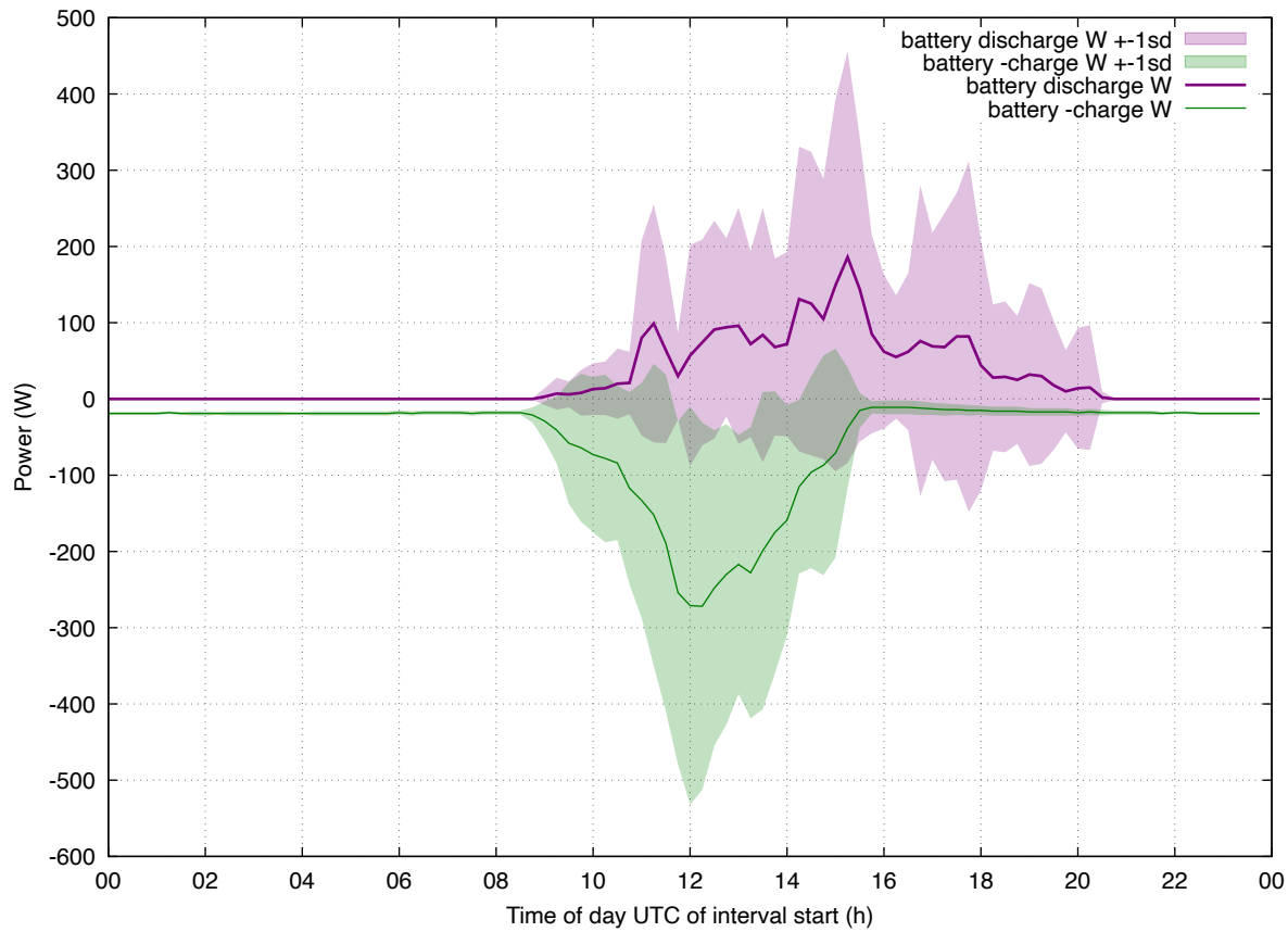
Load Profile: 202601 enphase-batt all
