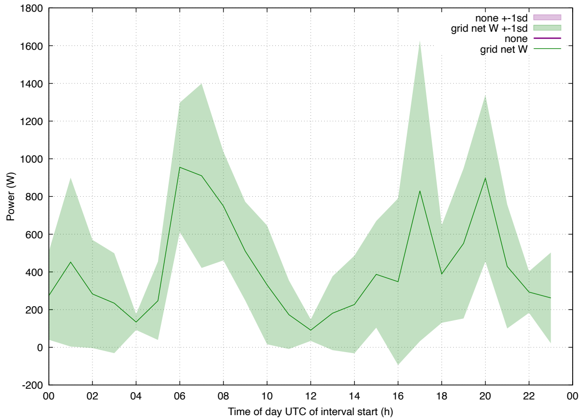
Load Profile: 202601 eddi weekend
