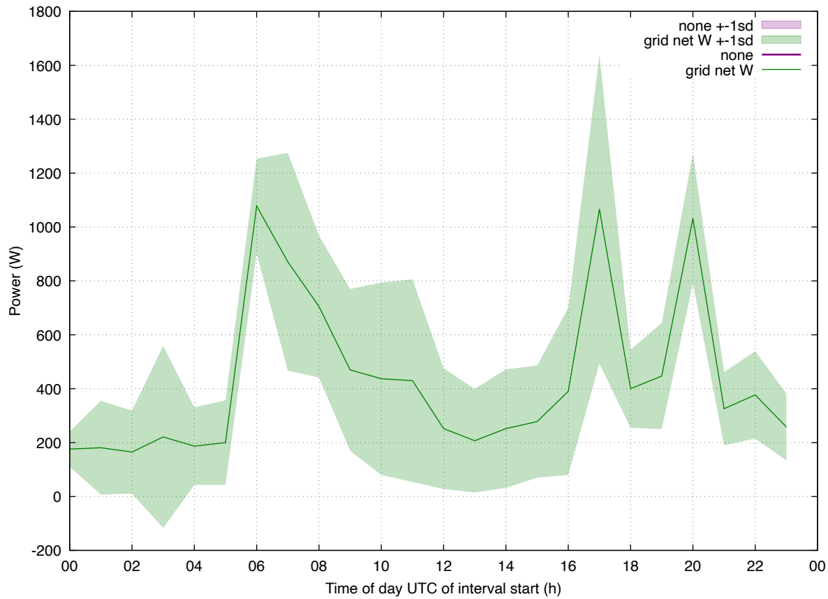
Load Profile: 202601 eddi weekday
