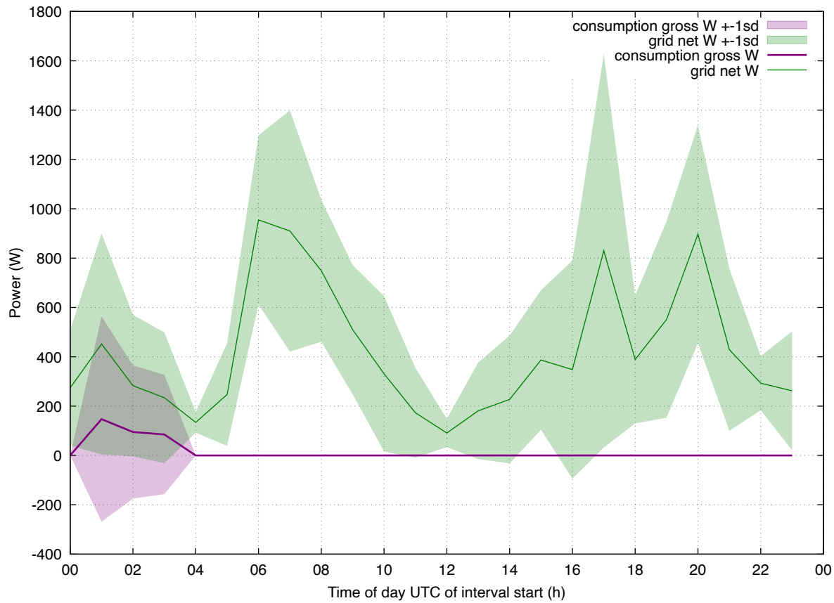
Load Profile: 202601 eddi-iheat weekend
