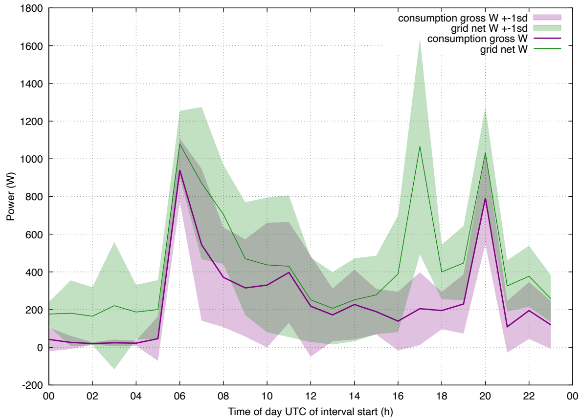
Load Profile: 202601 eddi-hph4 weekday
