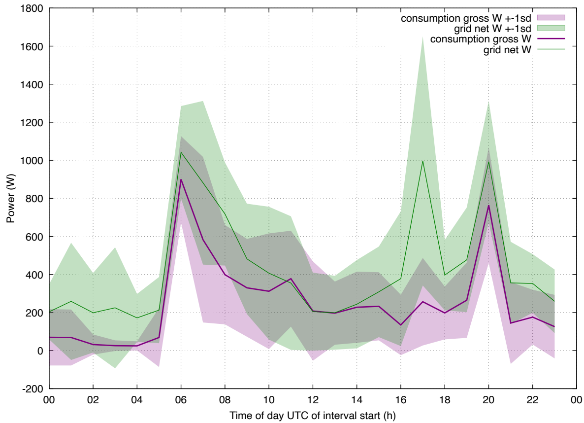
Load Profile: 202601 eddi-hph4 all
