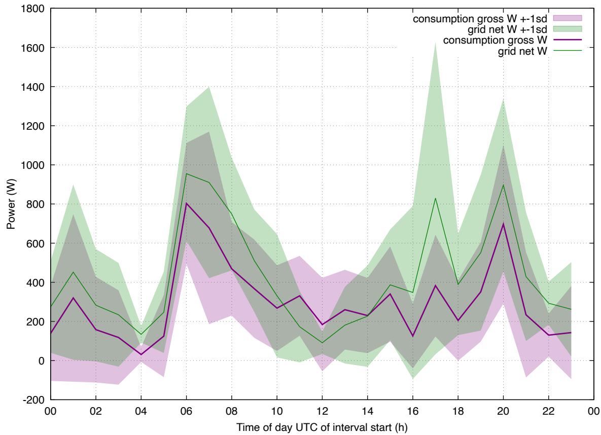
Load Profile: 202601 eddi-heat weekend
