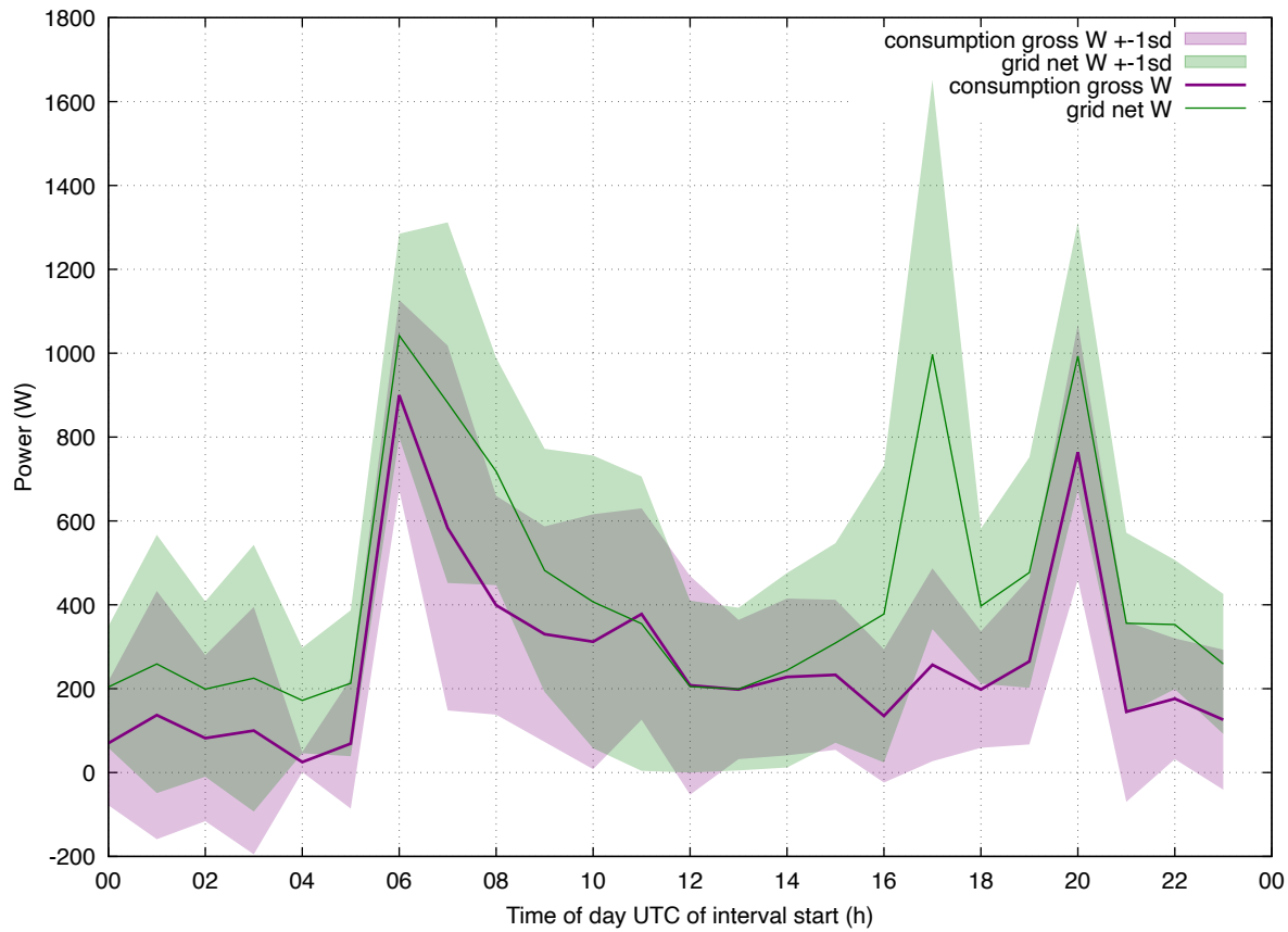
Load Profile: 202601 eddi-ehat all
