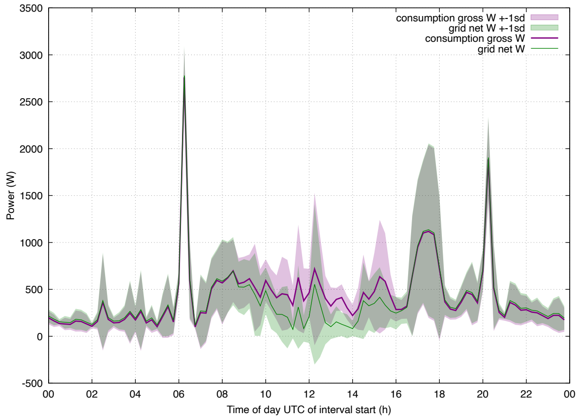
Load Profile: 202512 enphase weekend
