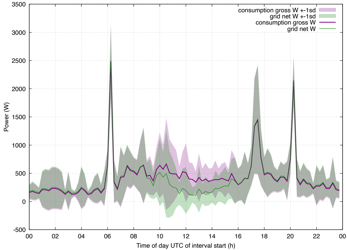
Load Profile: 202512 enphase weekday
