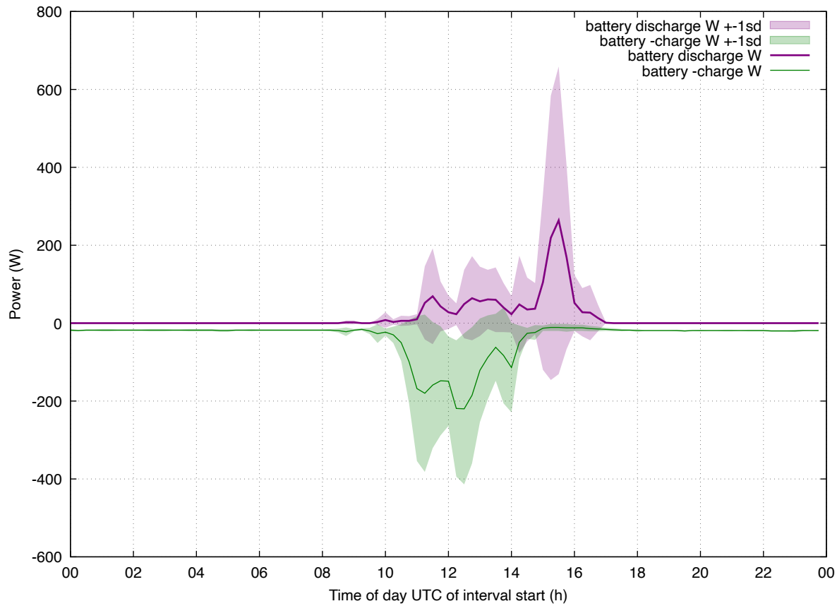
Load Profile: 202512 enphase-batt weekend
