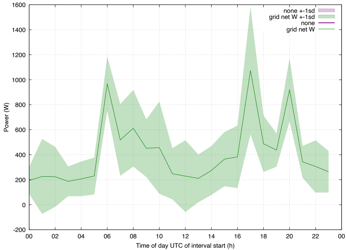
Load Profile: 202512 eddi all
