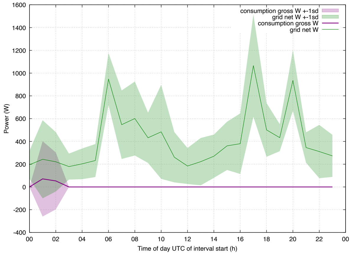
Load Profile: 202512 eddi-iheat weekday
