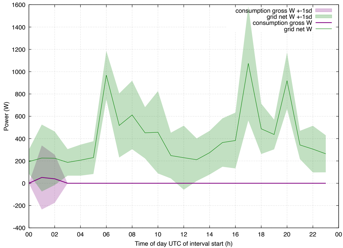
Load Profile: 202512 eddi-iheat all
