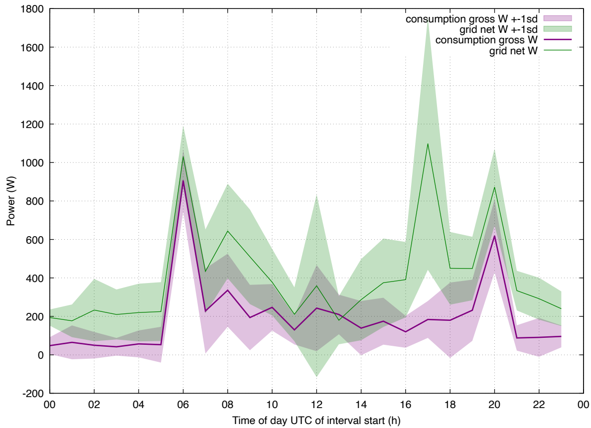
Load Profile: 202512 eddi-hph4 weekend
