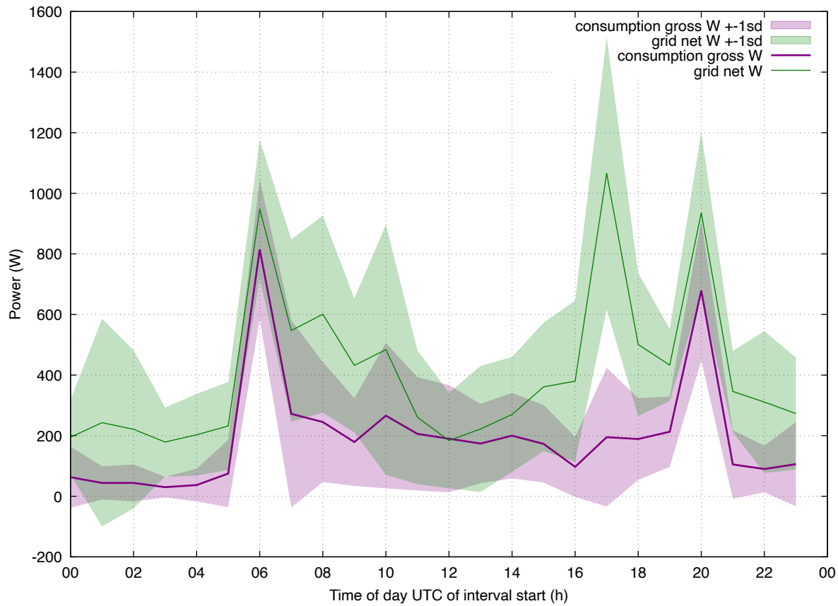
Load Profile: 202512 eddi-hph4 weekday
