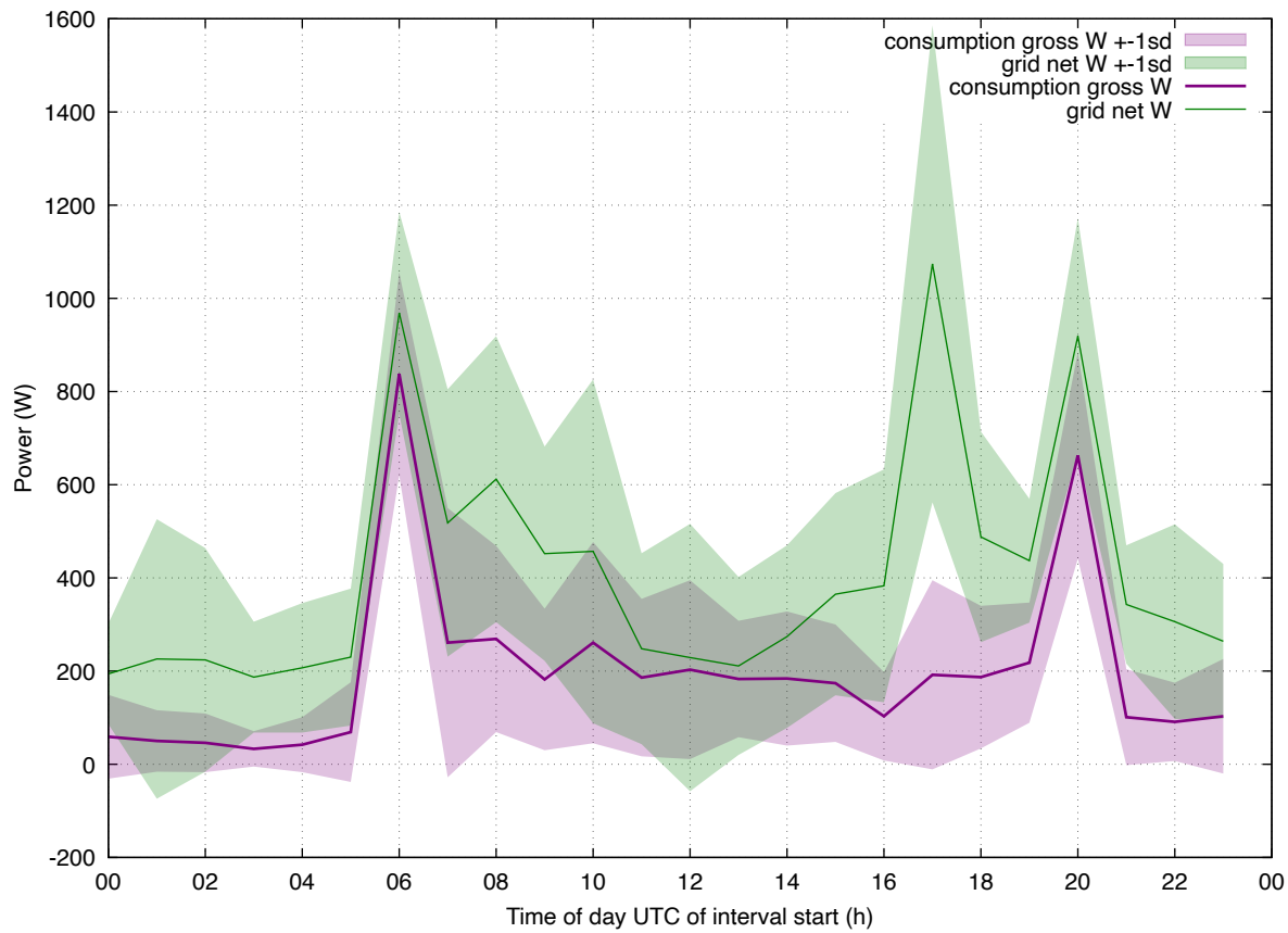
Load Profile: 202512 eddi-hph4 all
