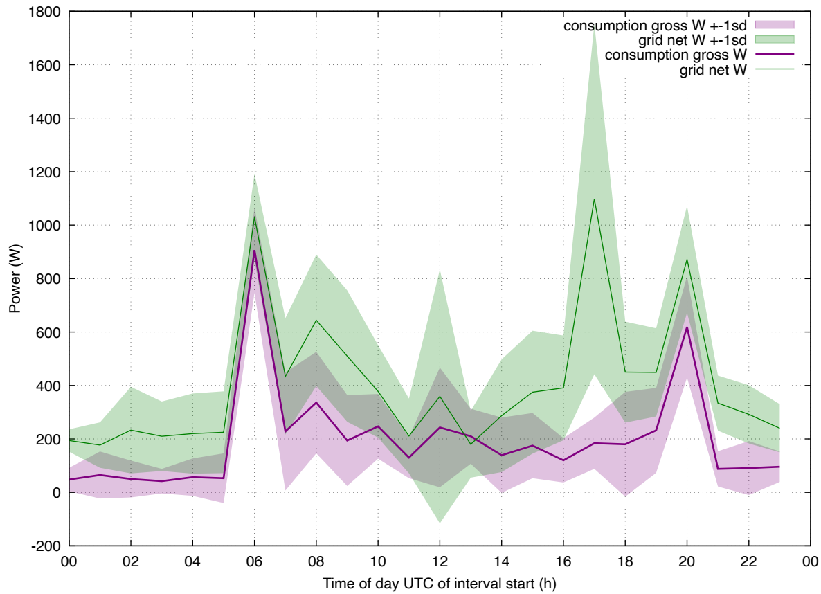
Load Profile: 202512 eddi-eheat weekend
