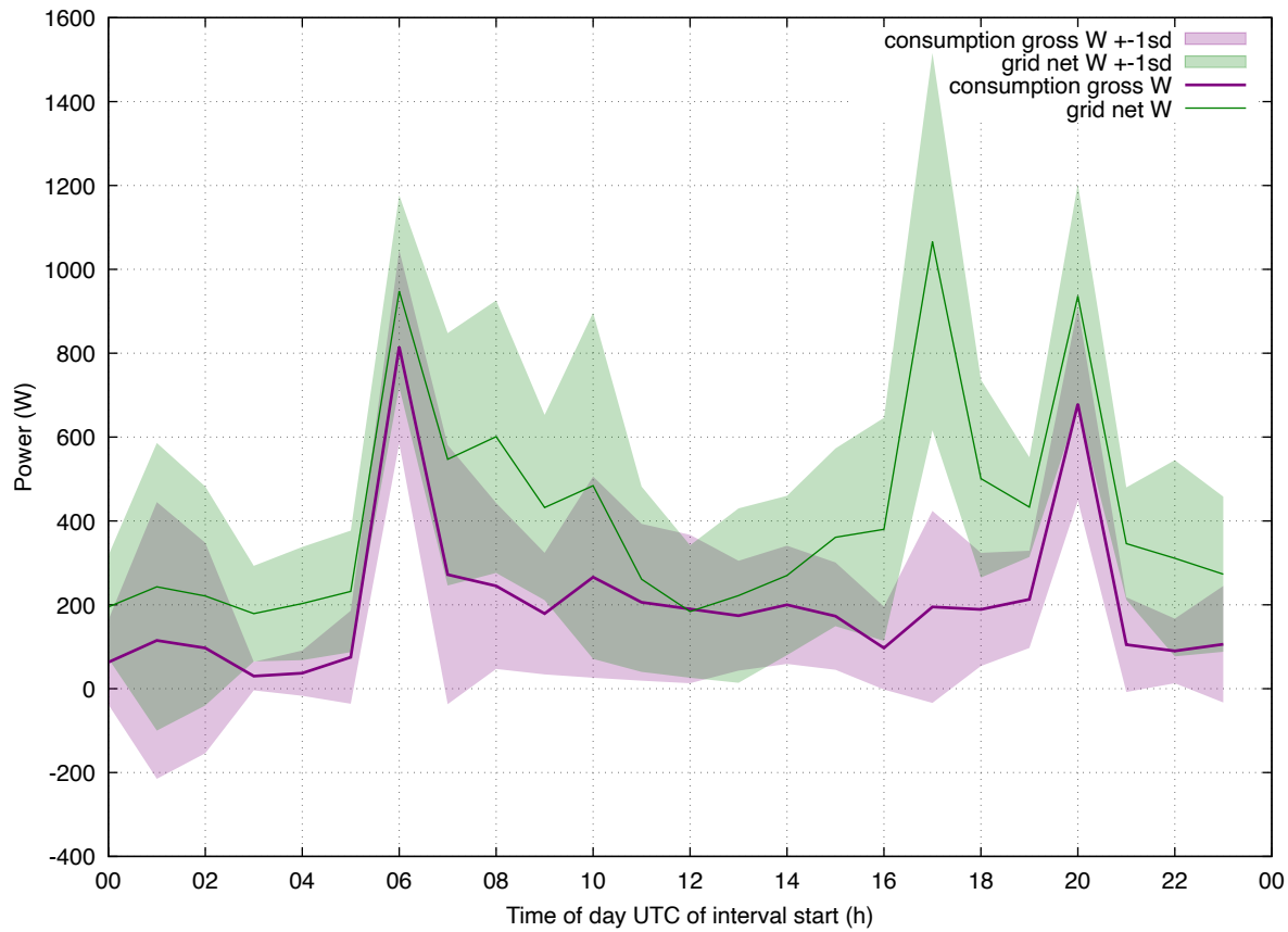
Load Profile: 202512 eddi-eheat weekday
