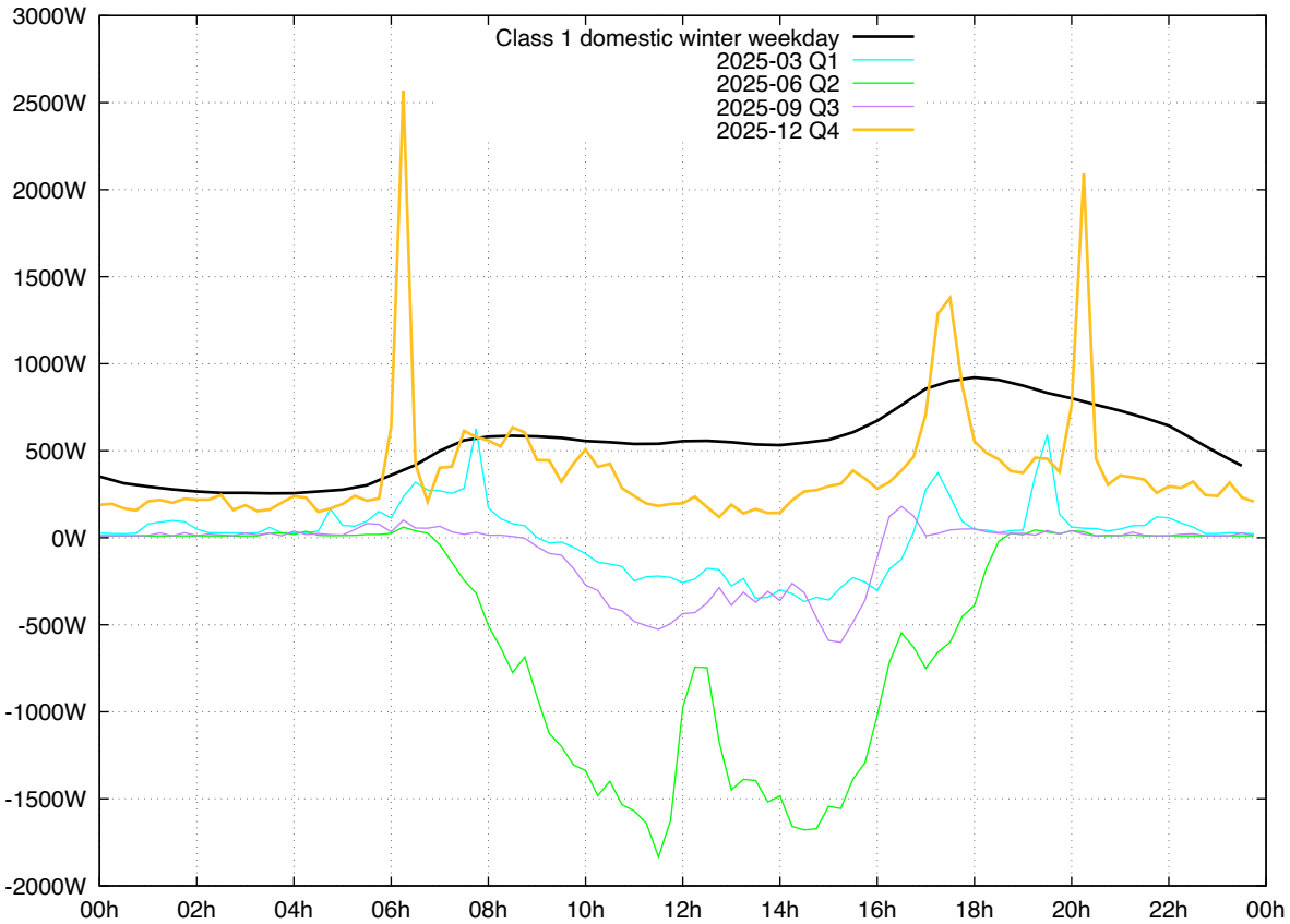
16WW Grid Net Load Profile 2025
